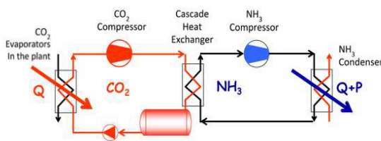
Figure 2: Two-stage Refrigeration system
