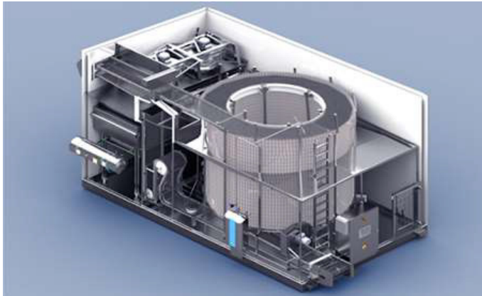
Figure 3: Spiral Freezer
